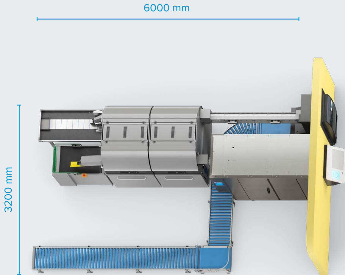
TOMRA R2+T9 with MultiPac, bottle raiser table, crossing crate line and SoftDrop
