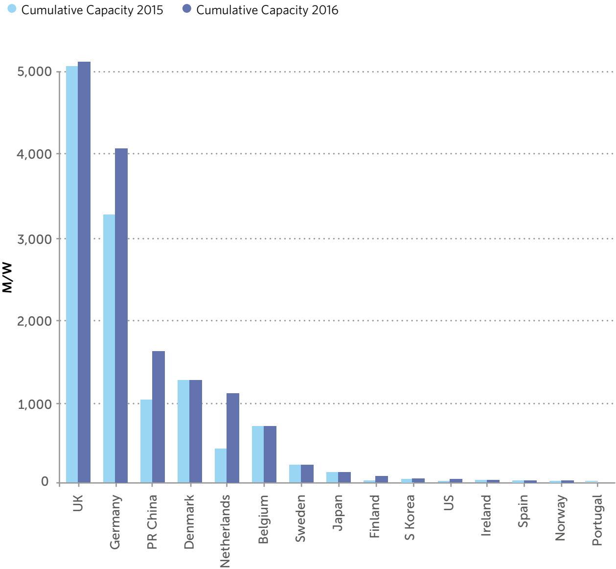
FIGURE 6 Global cumulative offshore wind capacity in 2016
